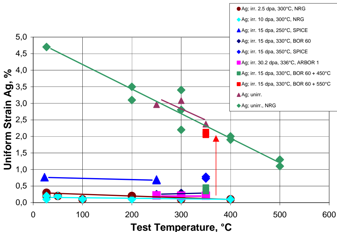
FIG. 9 Uniform Strain ( A_g ) behaviour of irradiated EUROFER 97 on dependence of test temperature compared to unirradiated data (the temperature in the legend indicates the irradiation temperature).
