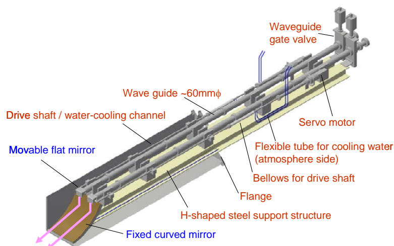
Fig. 14. Preliminary CAD model of the antenna for JT-60SA with reliable steering mirrors.
