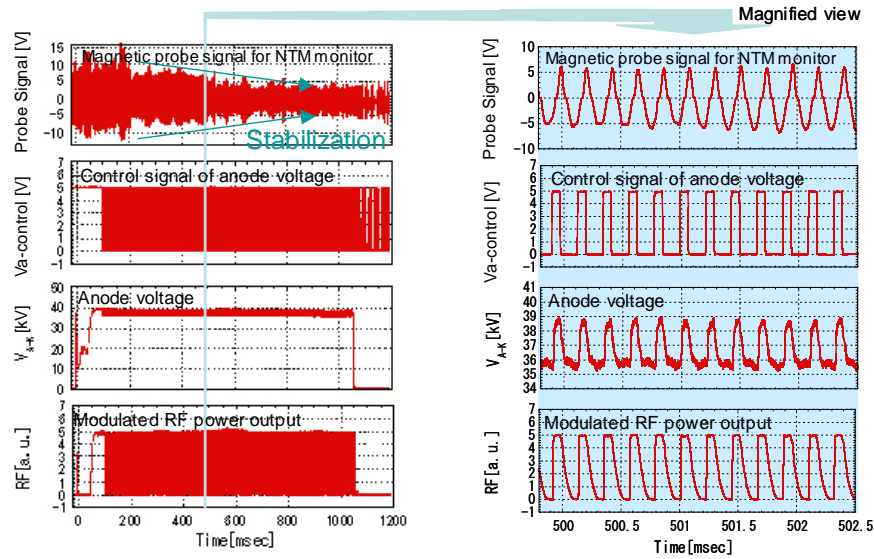
Fig. 10. Power modulation at \sim 5 kHz was achieved by controlling anode voltage for the NTM stabilization experiments. The modulation frequency and the phase was real-time-controlled referring to the magnetic probe as a reference of NTM oscillation.
