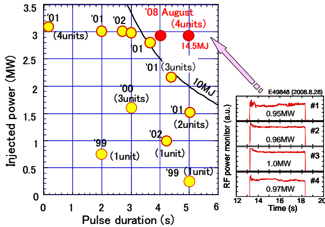
Fig. 1. Injected RF power and pulse duration of JT-60 ECRF system. Simultaneous operation of all 4 gyrotrons at 1MW for 5sec enabled 2.9 MW (14.5 MJ) injection with transmission efficiency of \sim 0.75 .
