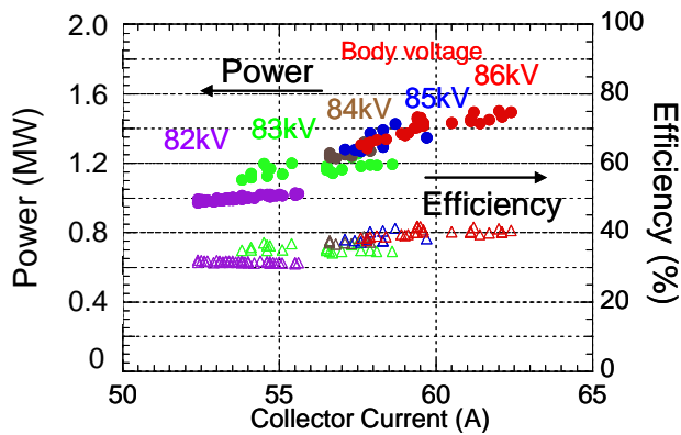
Fig. 5. Acceleration voltage and the collector current was raised carefully and gradually to obtain 1.5MW.
