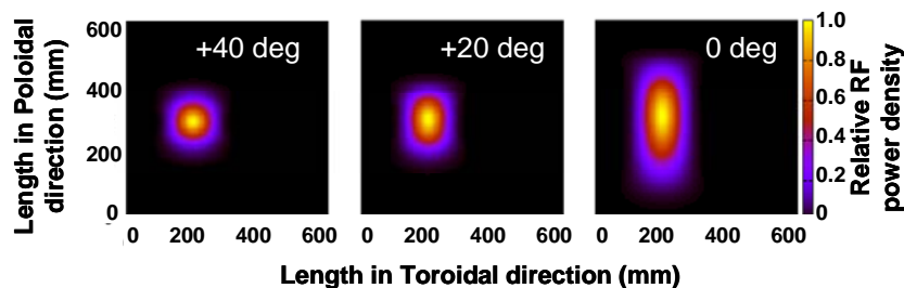
Fig. 12. Calculated beam power profiles at the typical poloidal injection angles.
