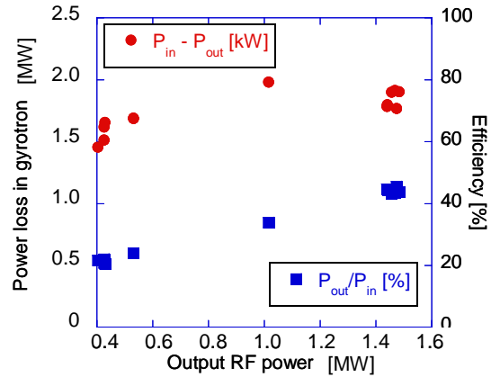
Fig.6. Gyrotron efficiency and power balance.
