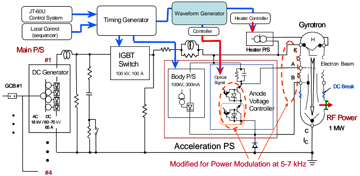
Fig. 9. Schematic diagram of power supply for long pulse gyrotron operation in JT-60U ECRF system.
