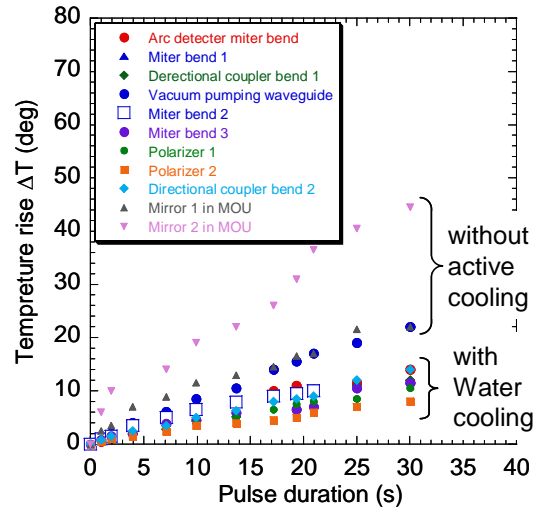
Fig. 8. Temperature rise of the each component in the transmission line. The peak of the temperature was measured during or just after the individual pulse, because thermocouple measurement has delay of a few seconds.
