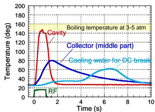
Fig. 4. Temperature of components in the gyrotron and cooling water on 1.5MW for 1s oscillation.
