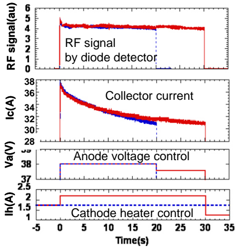
Fig. 7. Waveform of 0.4MW for 30s injection to the JT-60U plasma. Real time control of anode voltage and cathode-heater power was effective in keeping oscillation condition against the decay of collector current.
