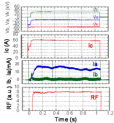
Fig. 2. Waveforms of high voltage applied to the gyrotron, current and RF signals on 1.5 MW for 1 s oscillation. The suffixes a, b, c, k stand for anode, body, collector and cathode respectively.
