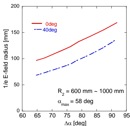
Fig. 13. Dependence of 1/e e-field radius on the range of poloidal beam angle.
