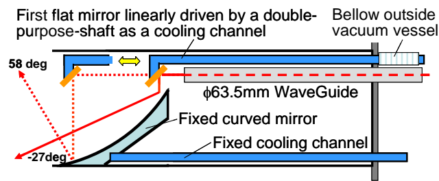
Fig. 11. Conceptual drawing of the antenna featuring a concept of “mirror driven in the linear motion”.
