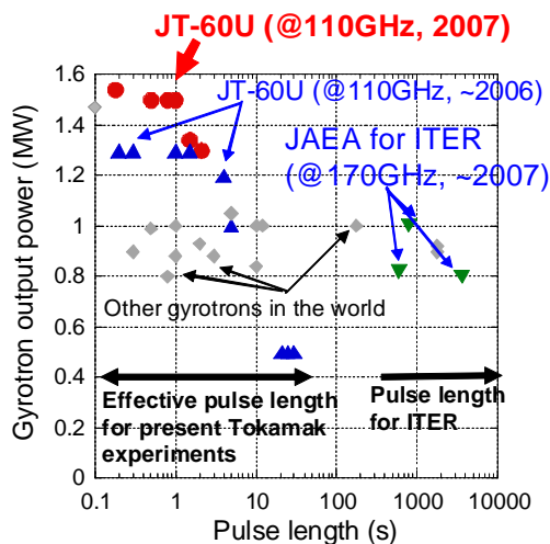
Fig. 3. Gyrotron output power achievements in the world for the pulse length of 0.1s or over.
